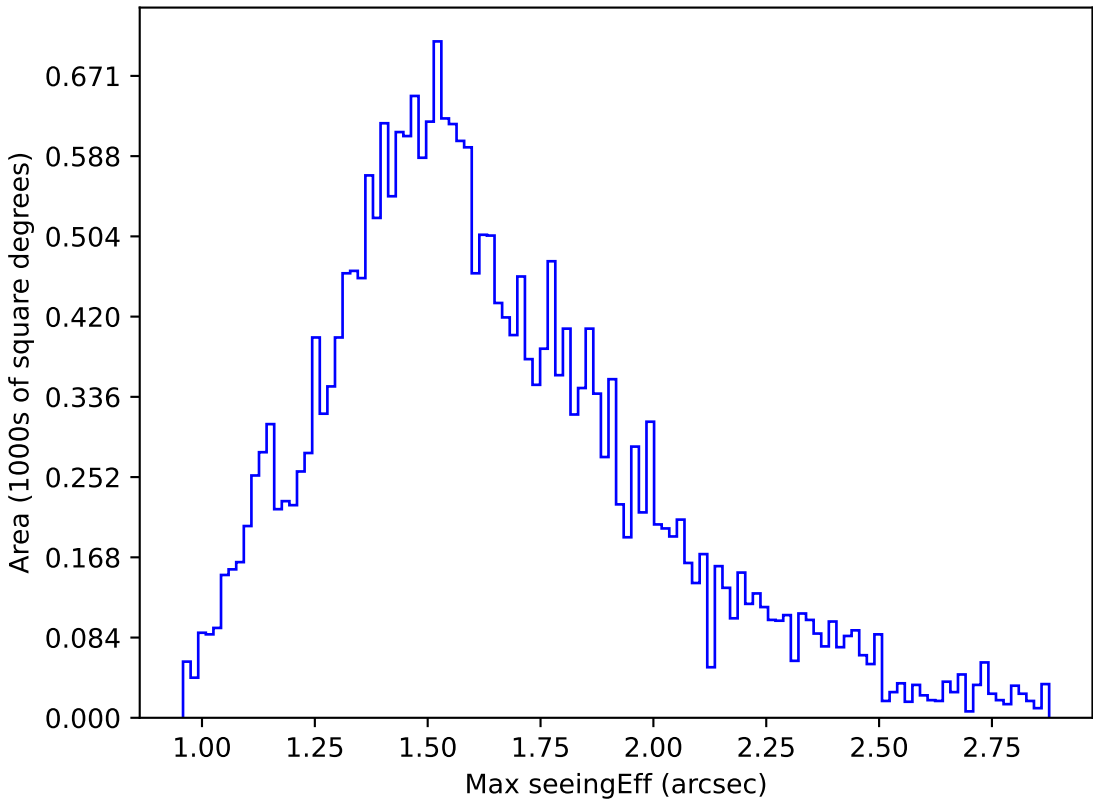
too_elab_r256_d2_griz_v3.4_10yrs Yr 1 r band: Max seeingEff
