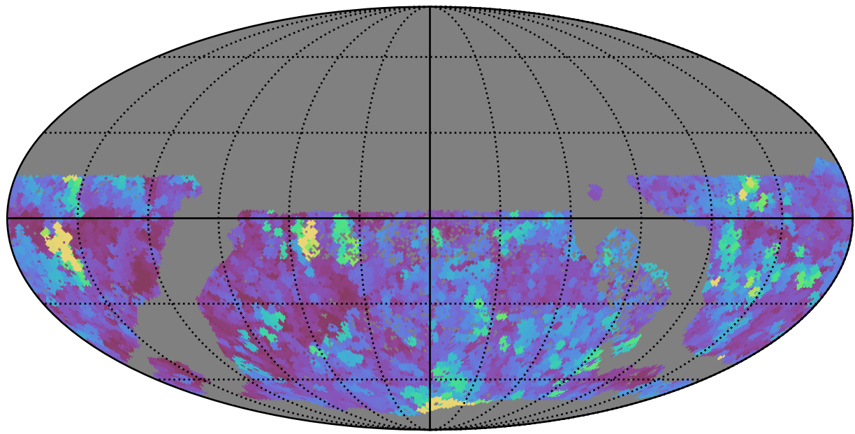
too_elab_r256_d2_griz_v3.4_10yrs WFD z band: Max seeingEff
