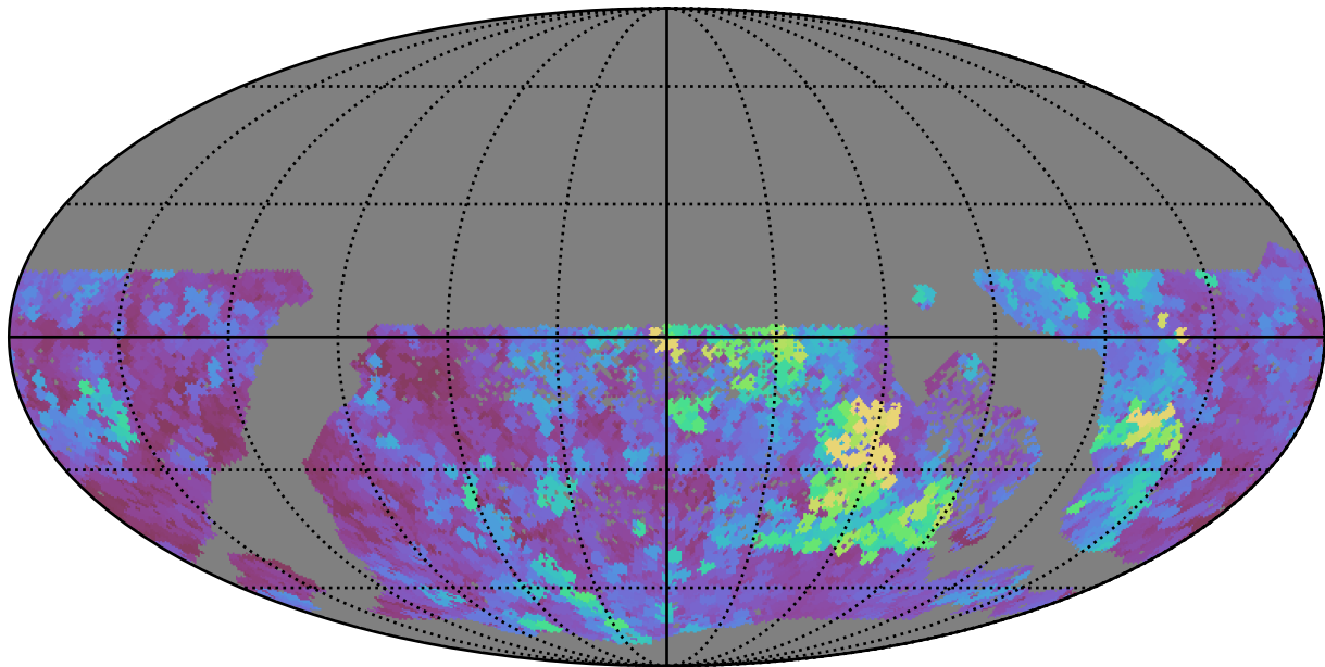
too_elab_r256_d2_griz_v3.4_10yrs WFD y band: Max seeingEff
