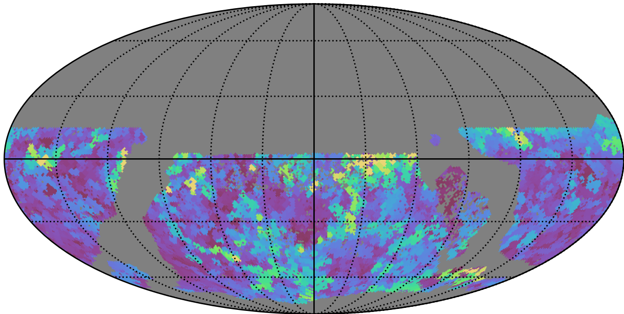
too_elab_r256_d2_griz_v3.4_10yrs WFD u band: Max seeingEff
