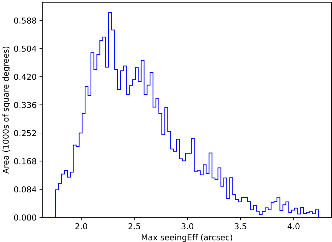
too_elab_r256_d2_griz_v3.4_10yrs WFD u band: Max seeingEff
