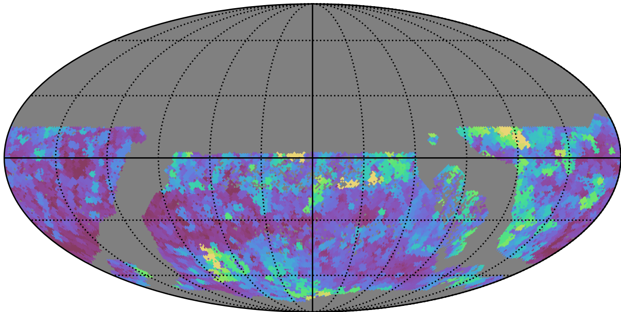
too_elab_r256_d2_griz_v3.4_10yrs WFD r band: Max seeingEff
