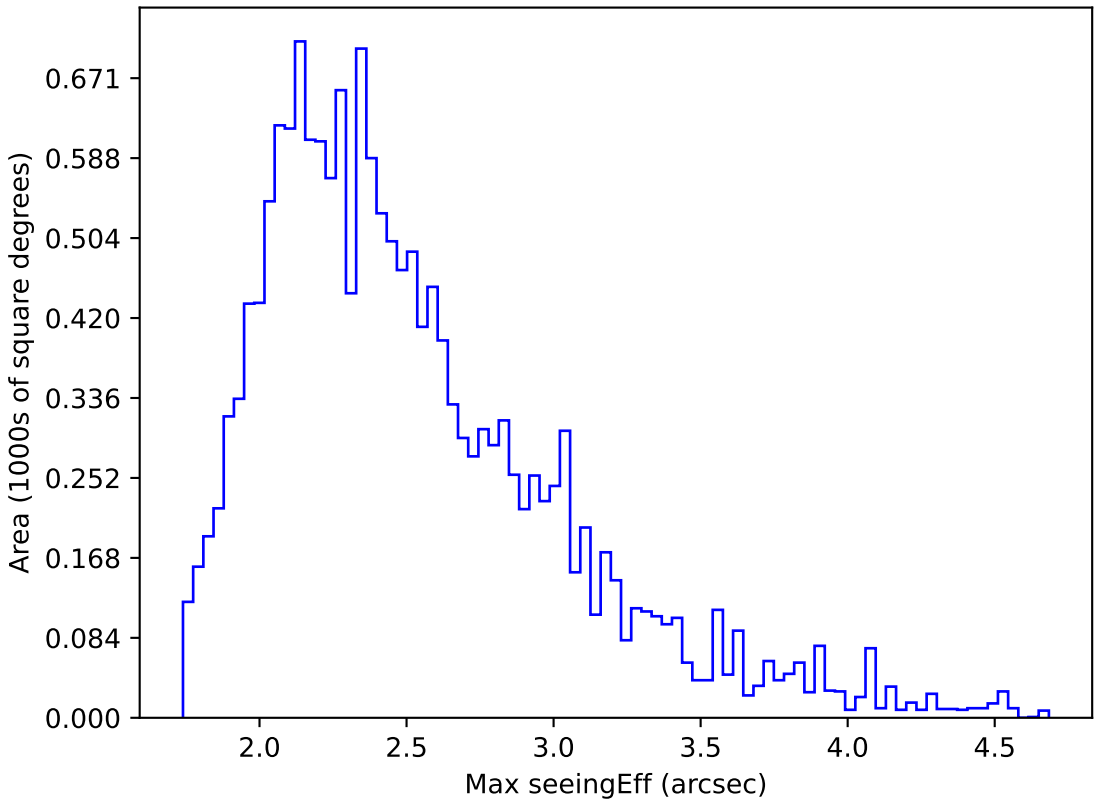
too_elab_r256_d2_griz_v3.4_10yrs WFD g band: Max seeingEff
