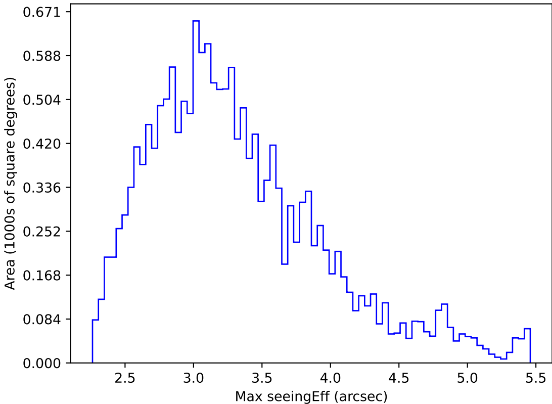
too_elab_r256_d2_griz_v3.4_10yrs WFD all bands: Max seeingEff
