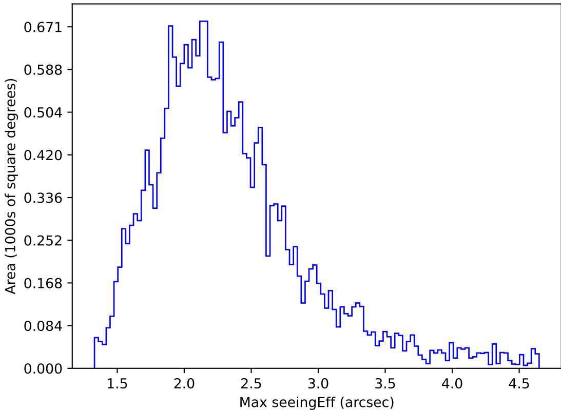
too_elab_r256_d2_griz_v3.4_10yrs All sky y band: Max seeingEff
