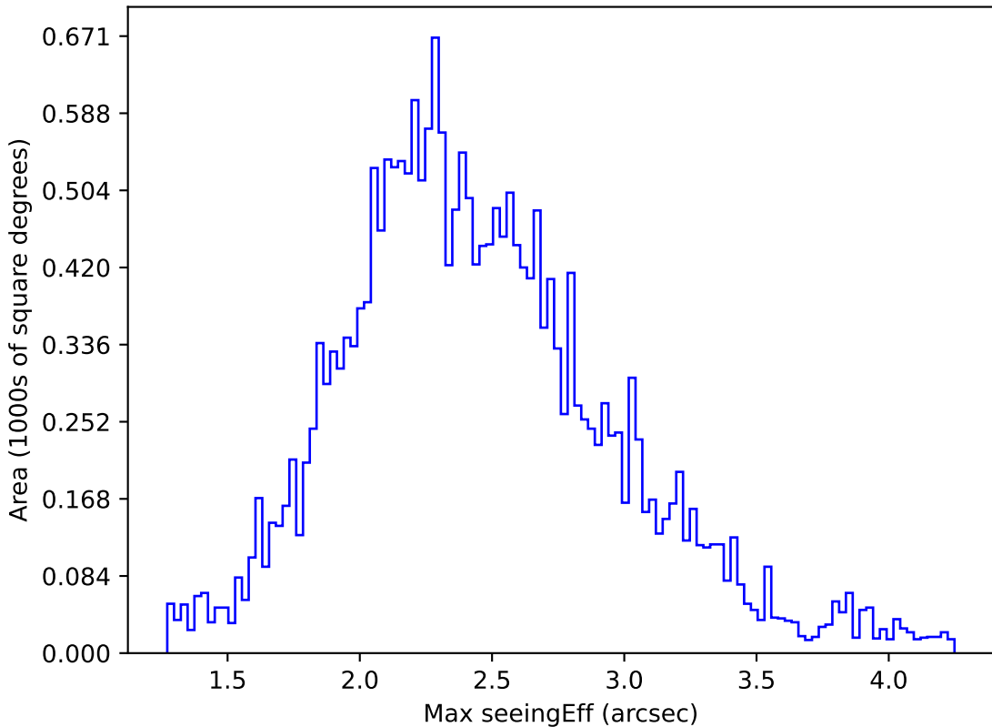
too_elab_r256_d2_griz_v3.4_10yrs All sky u band: Max seeingEff
