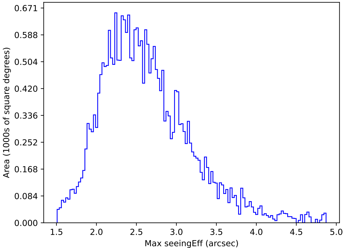
too_elab_r256_d2_griz_v3.4_10yrs All sky i band: Max seeingEff
