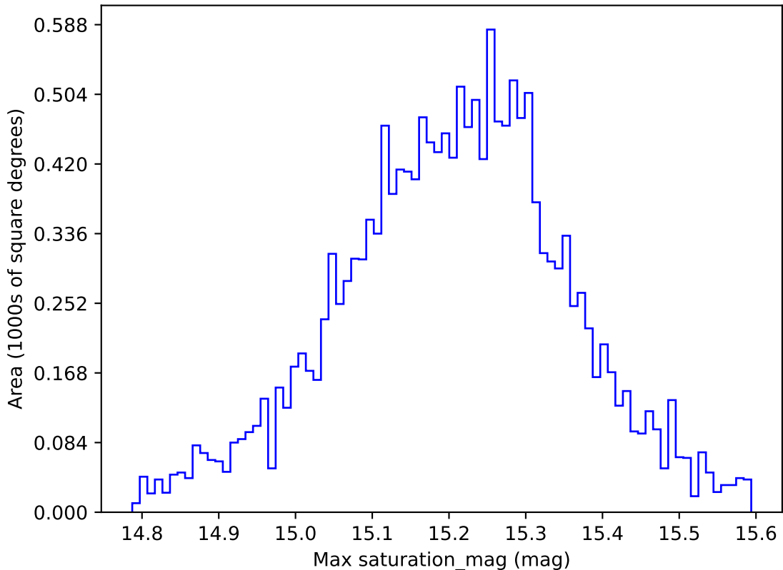
too_elab_r256_d2_griz_v3.4_10yrs WFD z band: Max saturation_mag
