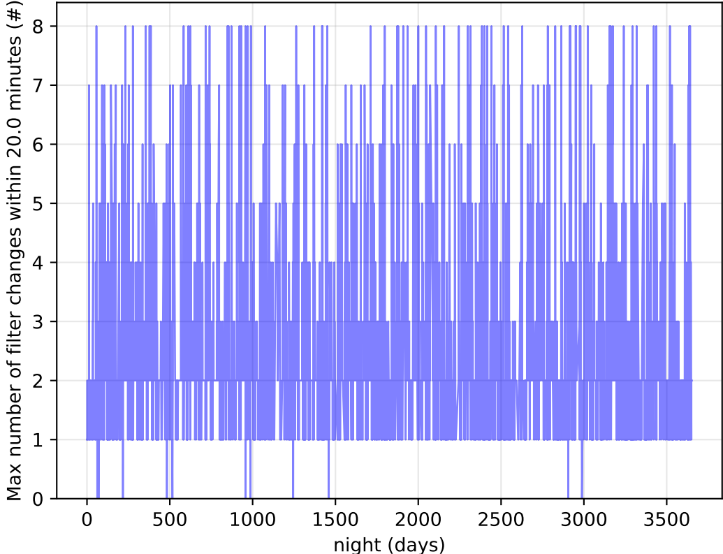
too_elab_r256_d2_griz_v3.4_10yrs Per Night: Max number of filter changes within 20.0 minutes
