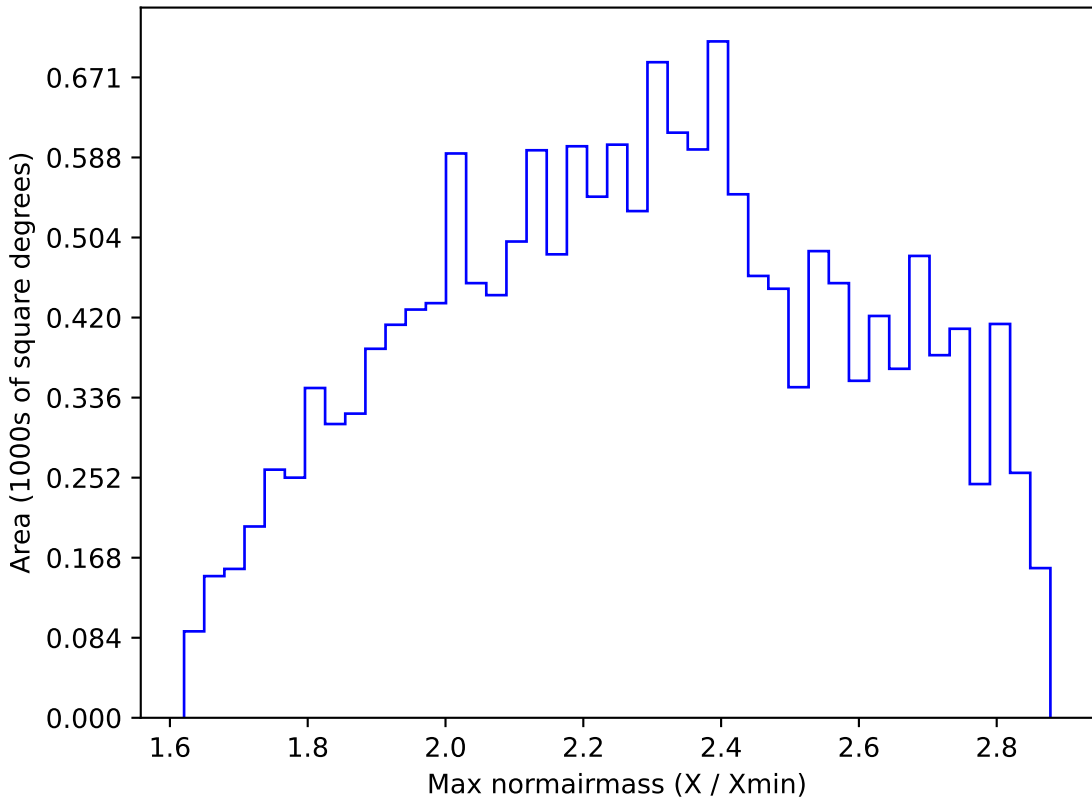
too_elab_r256_d2_griz_v3.4_10yrs WFD z band: Max normairmass
