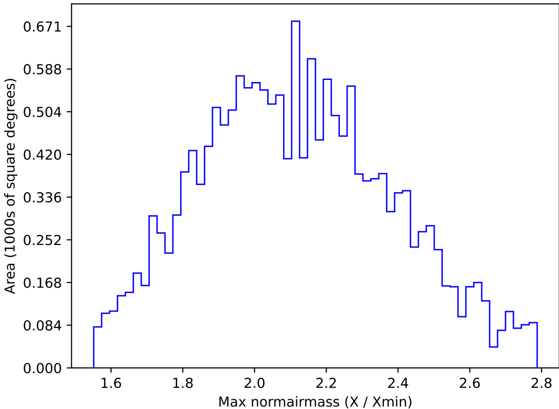
too_elab_r256_d2_griz_v3.4_10yrs WFD y band: Max normairmass
