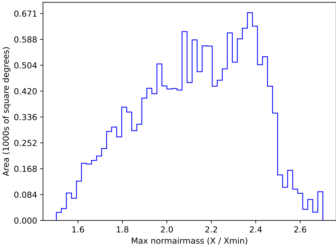
too_elab_r256_d2_griz_v3.4_10yrs WFD r band: Max normairmass
