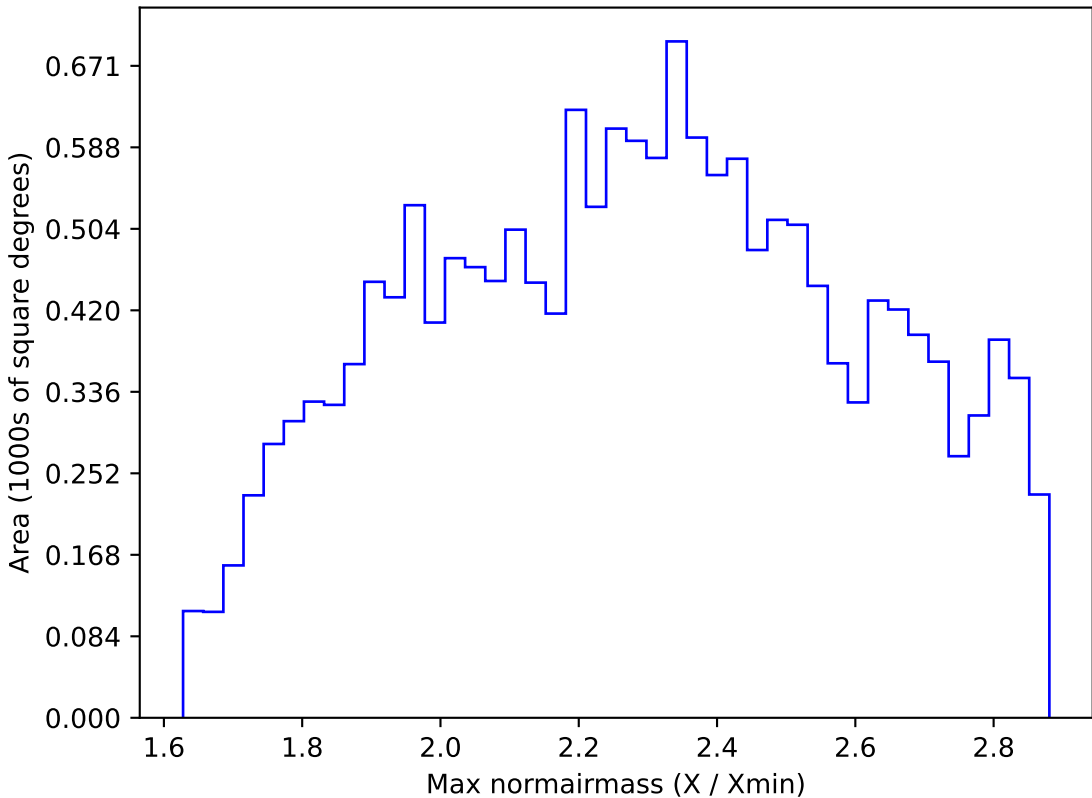
too_elab_r256_d2_griz_v3.4_10yrs WFD i band: Max normairmass
