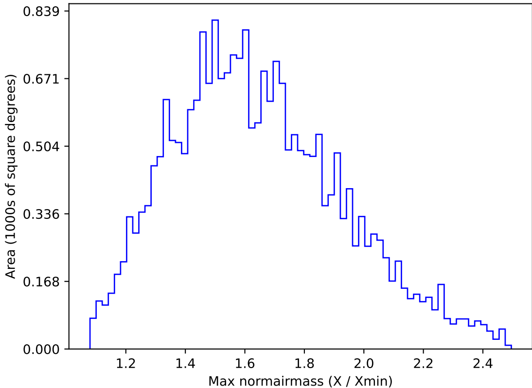
too_elab_r256_d2_griz_v3.4_10yrs All sky u band: Max normairmass
