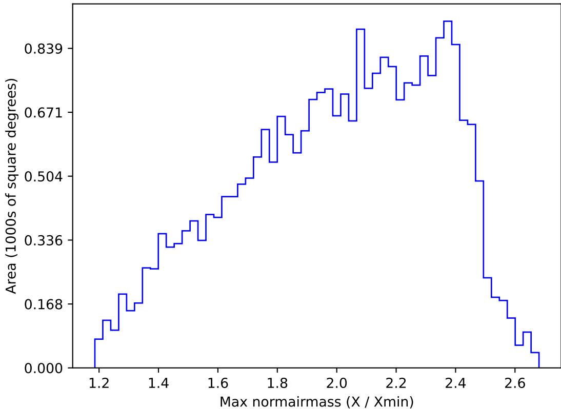
too_elab_r256_d2_griz_v3.4_10yrs All sky r band: Max normairmass
