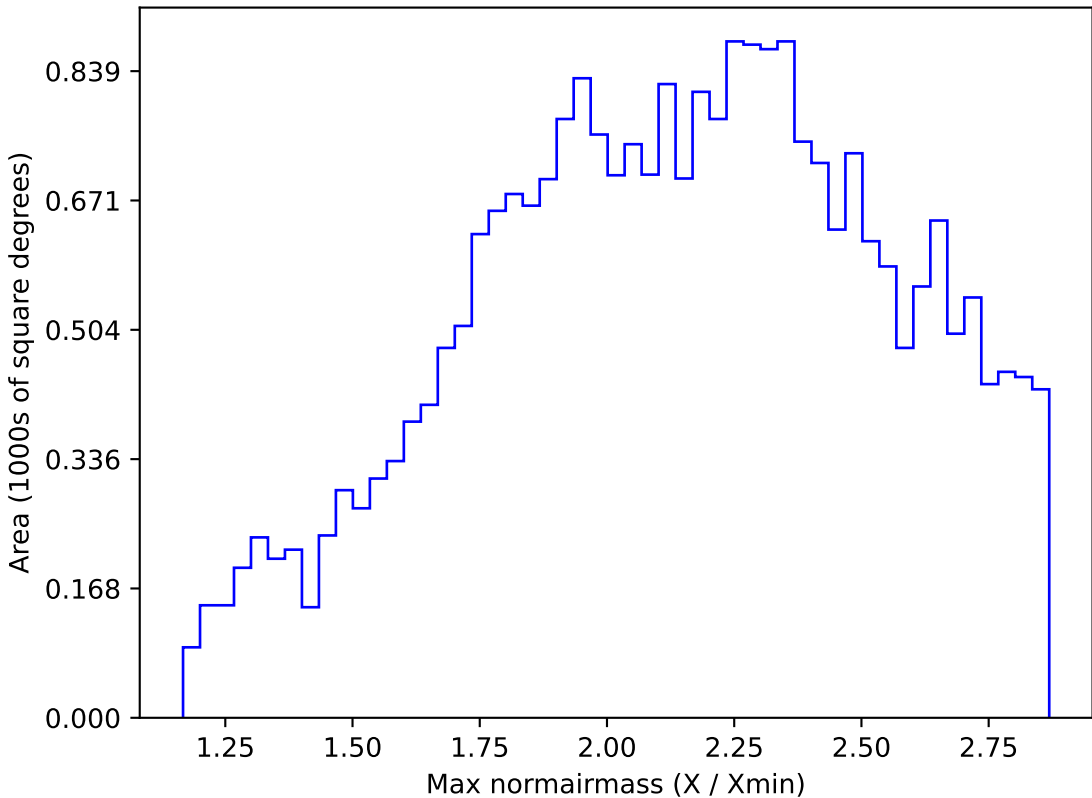
too_elab_r256_d2_griz_v3.4_10yrs All sky i band: Max normairmass
