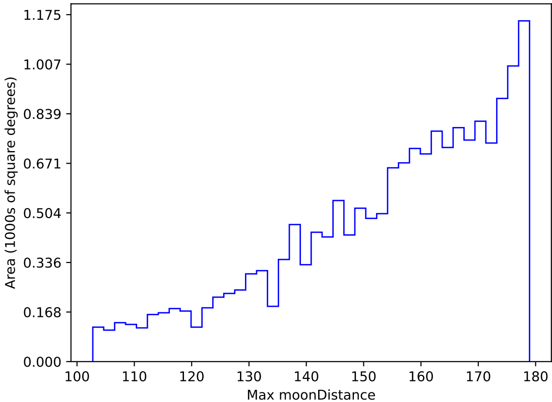
too_elab_r256_d2_griz_v3.4_10yrs WFD z band: Max moonDistance
