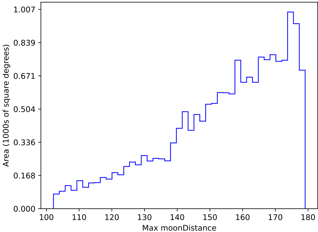
too_elab_r256_d2_griz_v3.4_10yrs WFD u band: Max moonDistance
