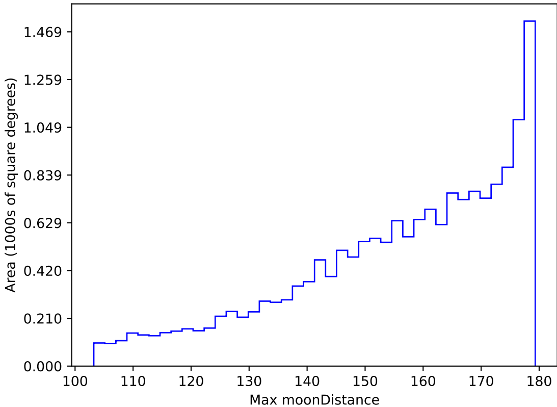
too_elab_r256_d2_griz_v3.4_10yrs WFD r band: Max moonDistance
