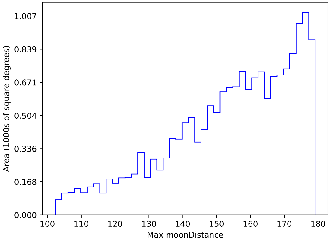
too_elab_r256_d2_griz_v3.4_10yrs WFD g band: Max moonDistance
