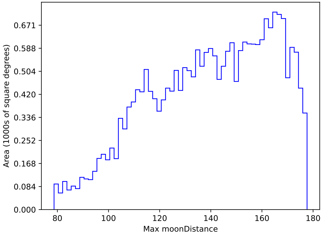
too_elab_r256_d2_griz_v3.4_10yrs All sky y band: Max moonDistance
