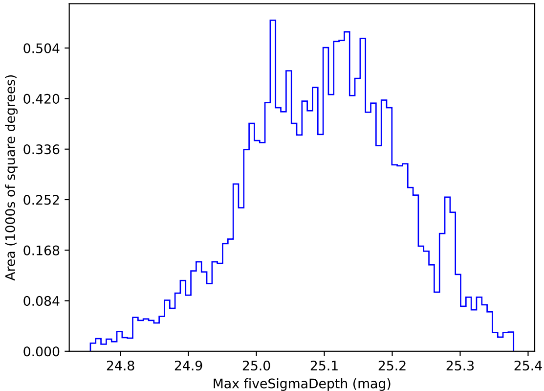
too_elab_r256_d2_griz_v3.4_10yrs WFD g band: Max fiveSigmaDepth
