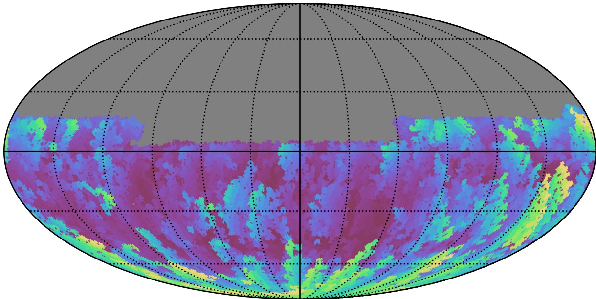
too_elab_r256_d2_griz_v3.4_10yrs Yr 1 u band: Max airmass
