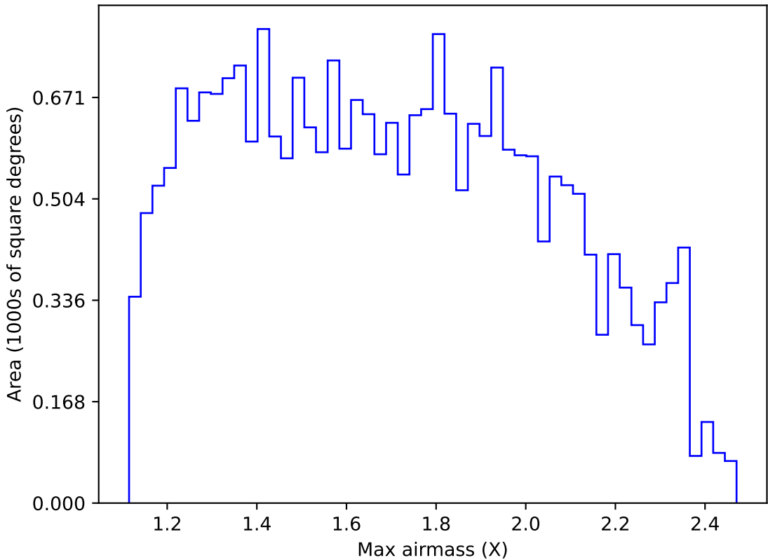
too_elab_r256_d2_griz_v3.4_10yrs Yr 1 g band: Max airmass
