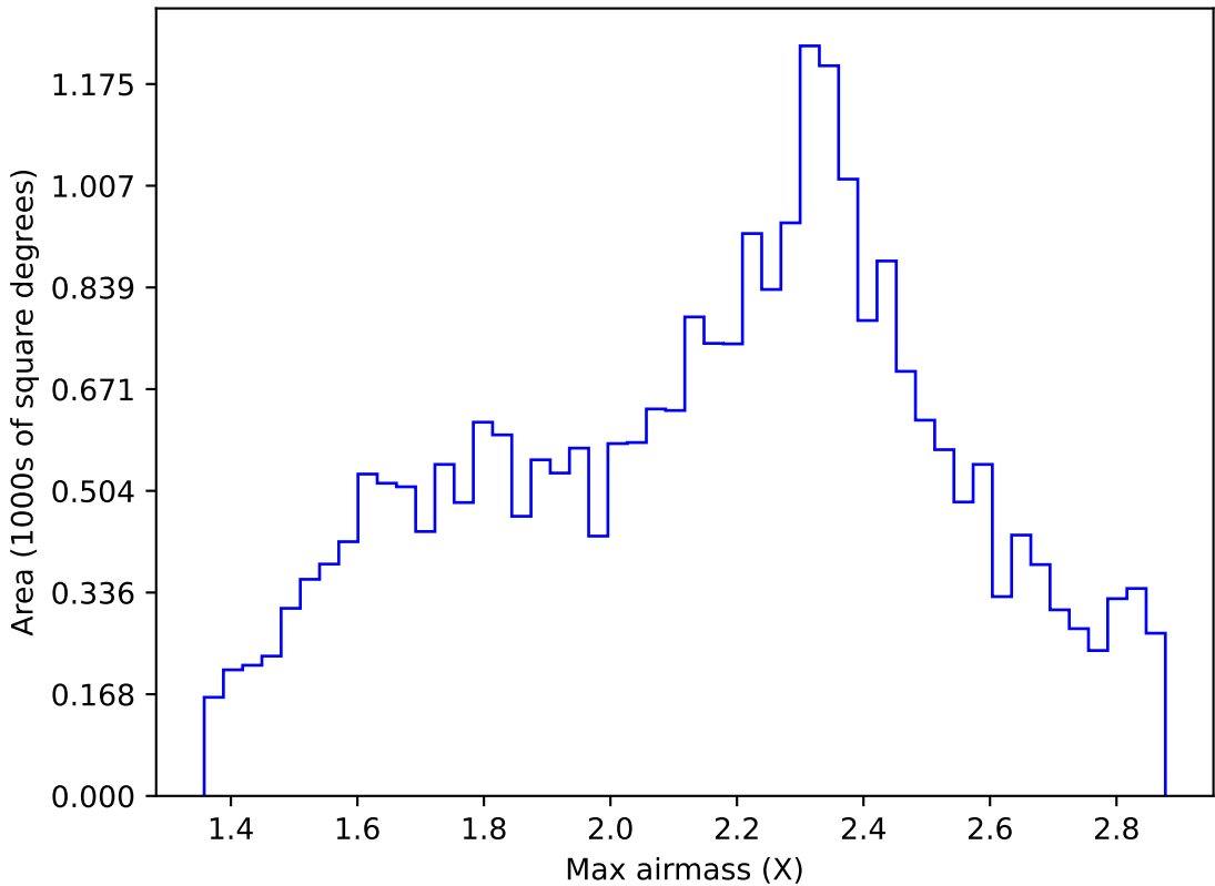
too_elab_r256_d2_griz_v3.4_10yrs Yr 1 all bands: Max airmass
