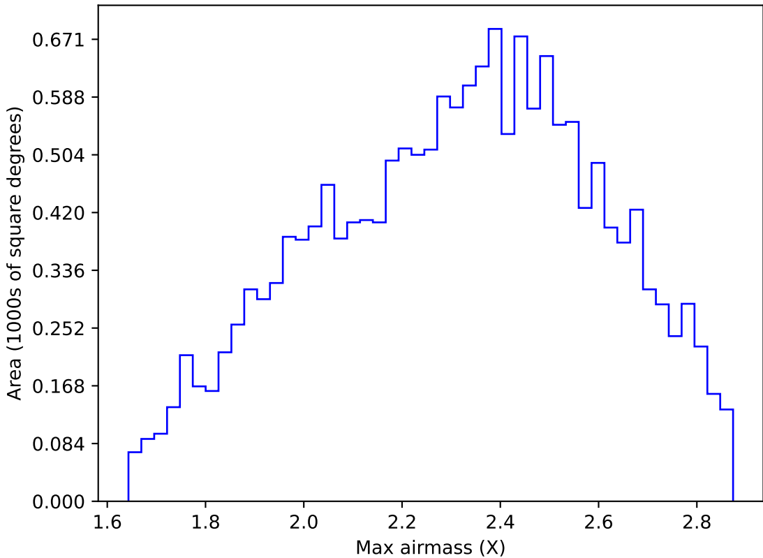
too_elab_r256_d2_griz_v3.4_10yrs WFD y band: Max airmass
