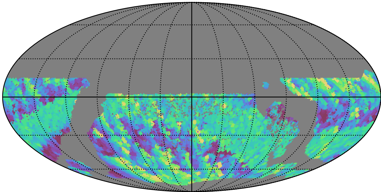
too_elab_r256_d2_griz_v3.4_10yrs WFD r band: Max airmass
