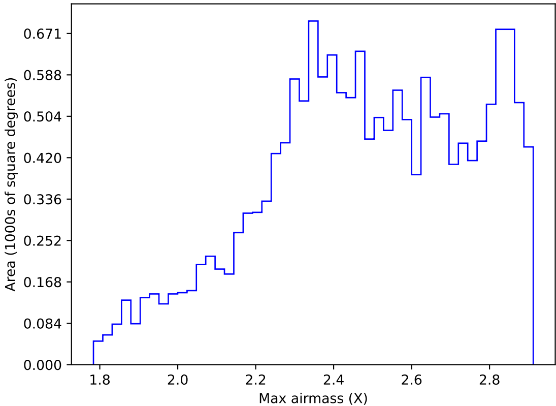
too_elab_r256_d2_griz_v3.4_10yrs WFD i band: Max airmass
