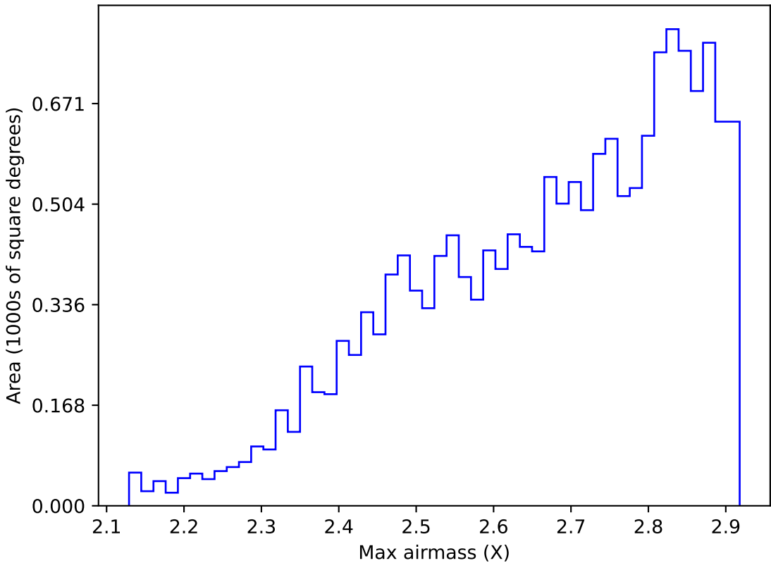
too_elab_r256_d2_griz_v3.4_10yrs WFD all bands: Max airmass
