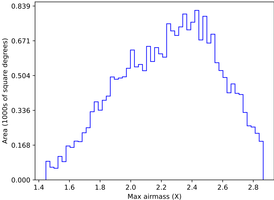
too_elab_r256_d2_griz_v3.4_10yrs All sky y band: Max airmass
