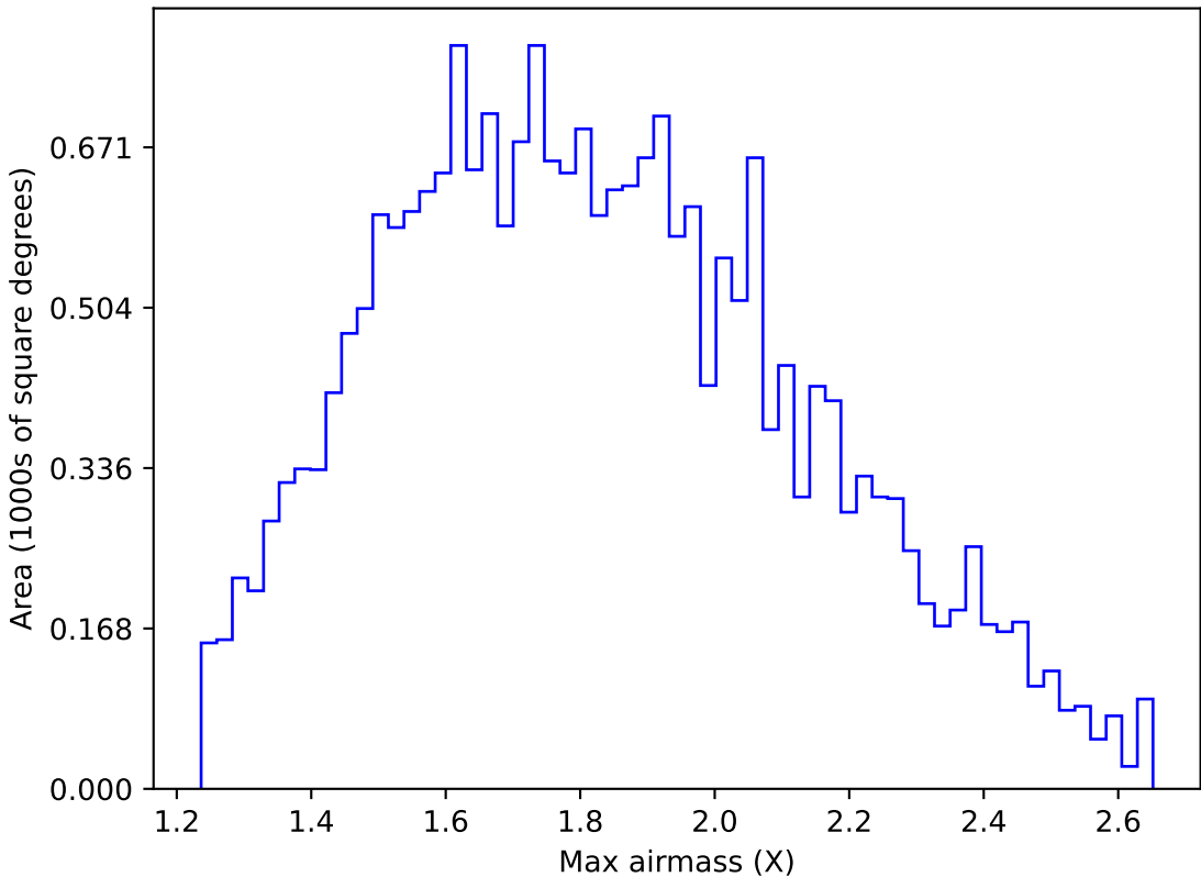
too_elab_r256_d2_griz_v3.4_10yrs All sky u band: Max airmass
