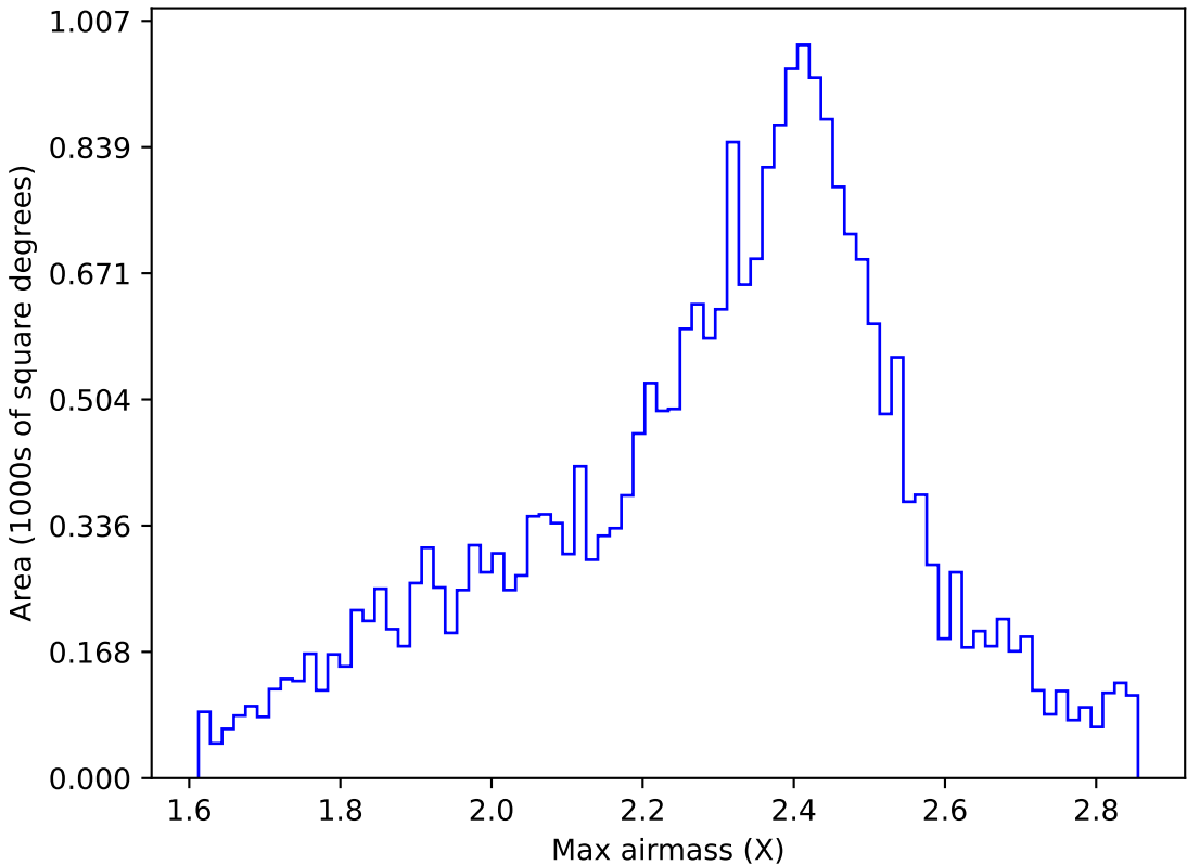
too_elab_r256_d2_griz_v3.4_10yrs All sky r band: Max airmass
