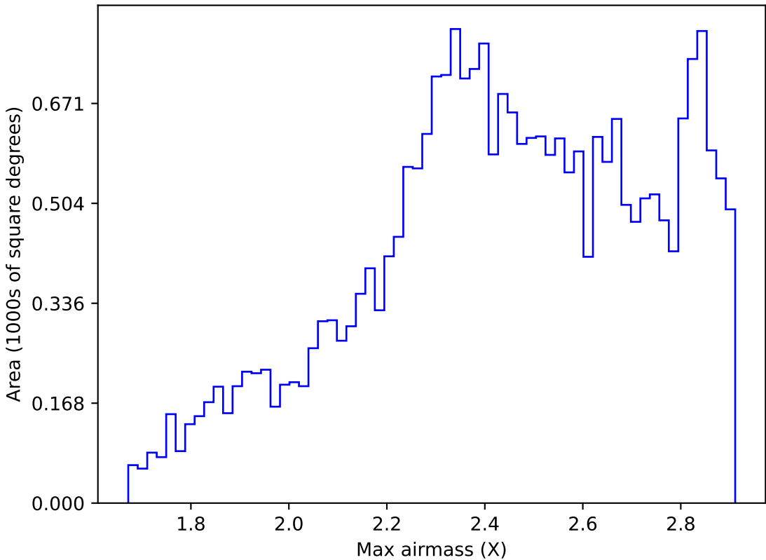
too_elab_r256_d2_griz_v3.4_10yrs All sky i band: Max airmass
