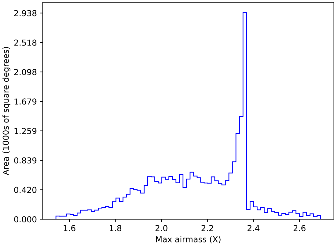
too_elab_r256_d2_griz_v3.4_10yrs All sky g band: Max airmass
