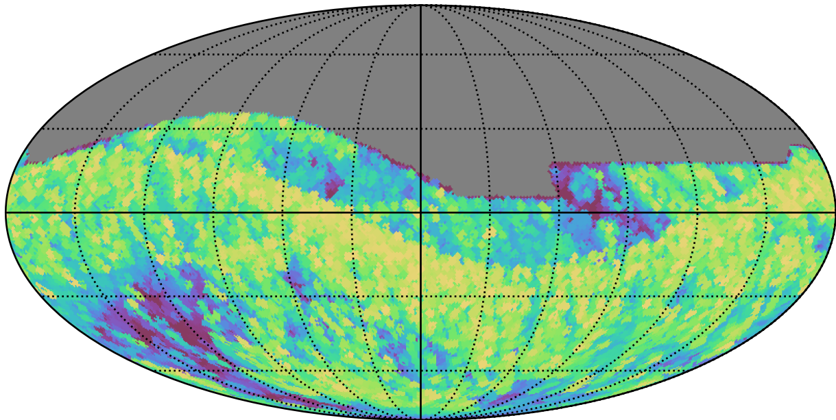
too_elab_r256_d2_griz_v3.4_10yrs All sky all bands: Max airmass
