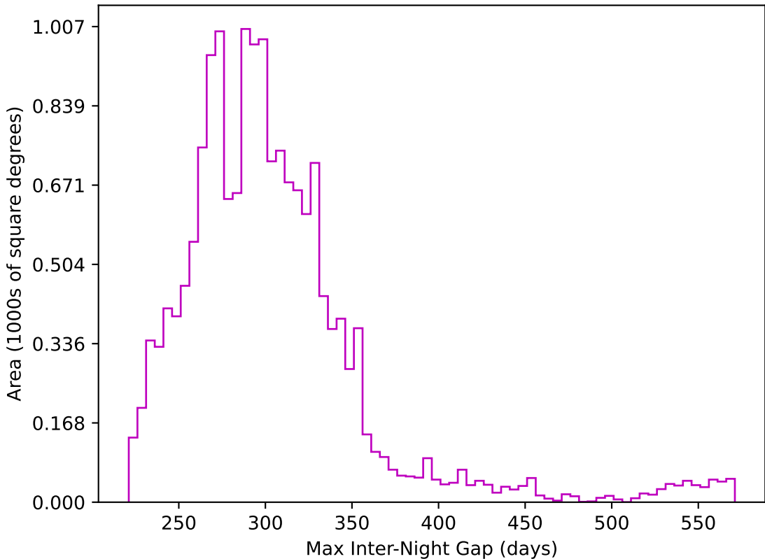
too_elab_r256_d2_griz_v3.4_10yrs WFD z band: Max Inter-Night Gap
