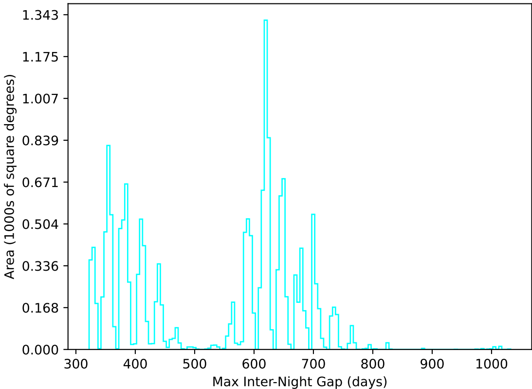
too_elab_r256_d2_griz_v3.4_10yrs WFD u band: Max Inter-Night Gap
