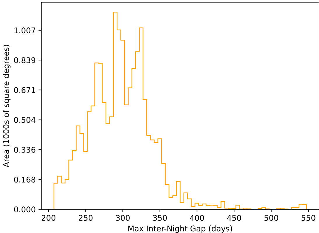
too_elab_r256_d2_griz_v3.4_10yrs WFD r band: Max Inter-Night Gap
