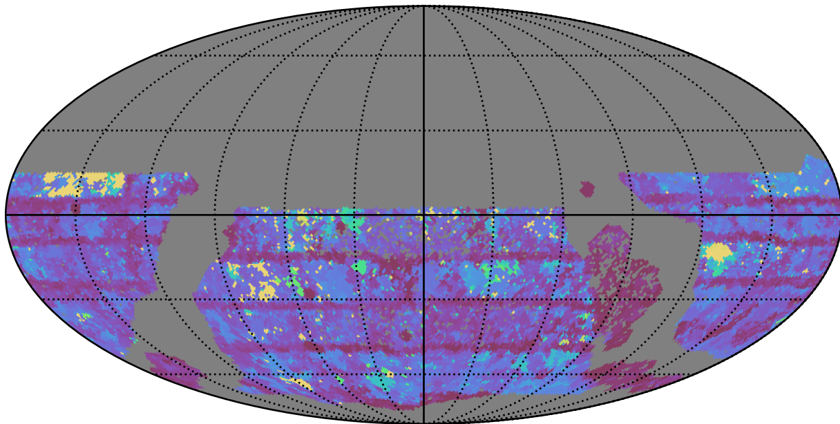
too_elab_r256_d2_griz_v3.4_10yrs WFD i band: Max Inter-Night Gap
