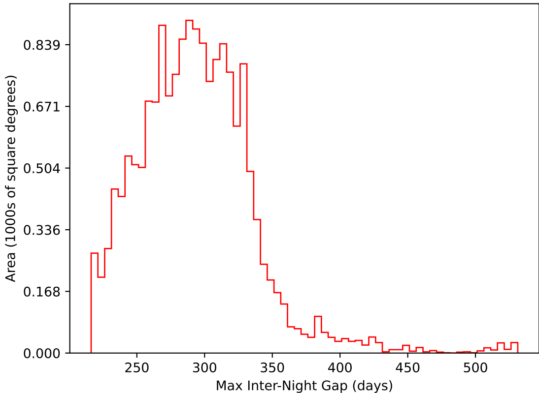
too_elab_r256_d2_griz_v3.4_10yrs WFD i band: Max Inter-Night Gap
