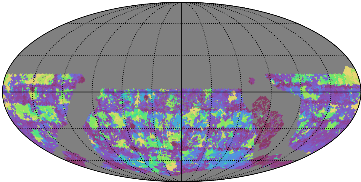
too_elab_r256_d2_griz_v3.4_10yrs WFD g band: Max Inter-Night Gap
