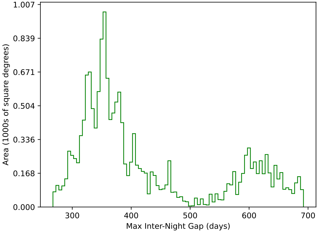
too_elab_r256_d2_griz_v3.4_10yrs WFD g band: Max Inter-Night Gap
