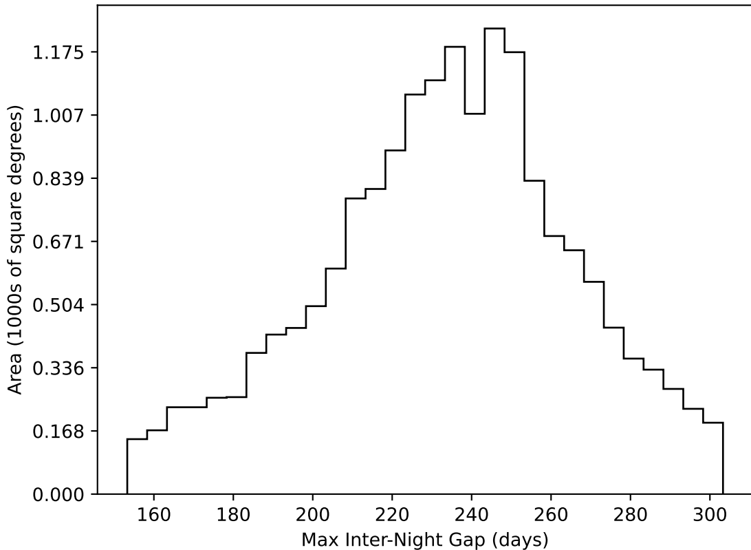
too_elab_r256_d2_griz_v3.4_10yrs WFD all bands: Max Inter-Night Gap
