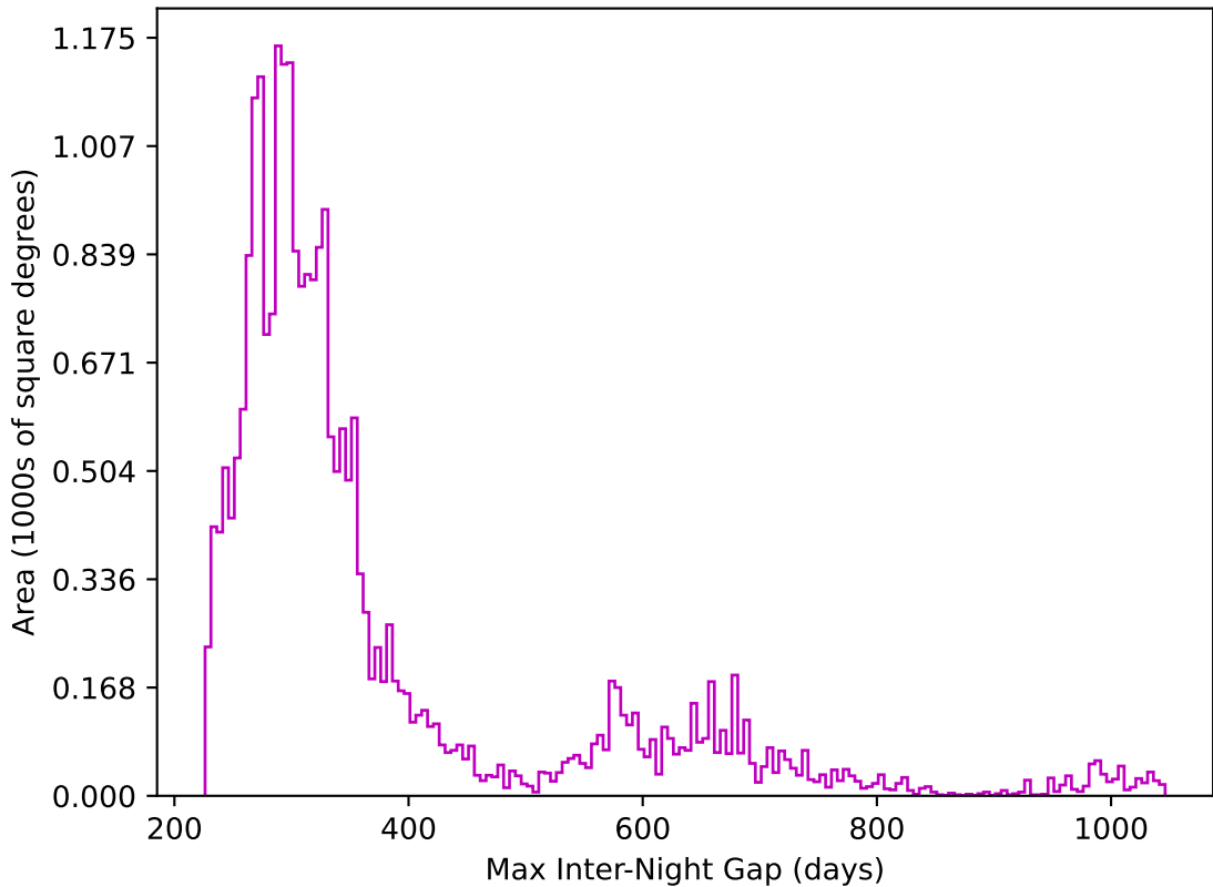
too_elab_r256_d2_griz_v3.4_10yrs All sky z band: Max Inter-Night Gap
