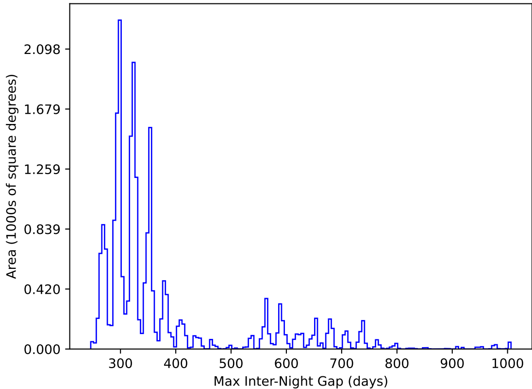
too_elab_r256_d2_griz_v3.4_10yrs All sky y band: Max Inter-Night Gap
