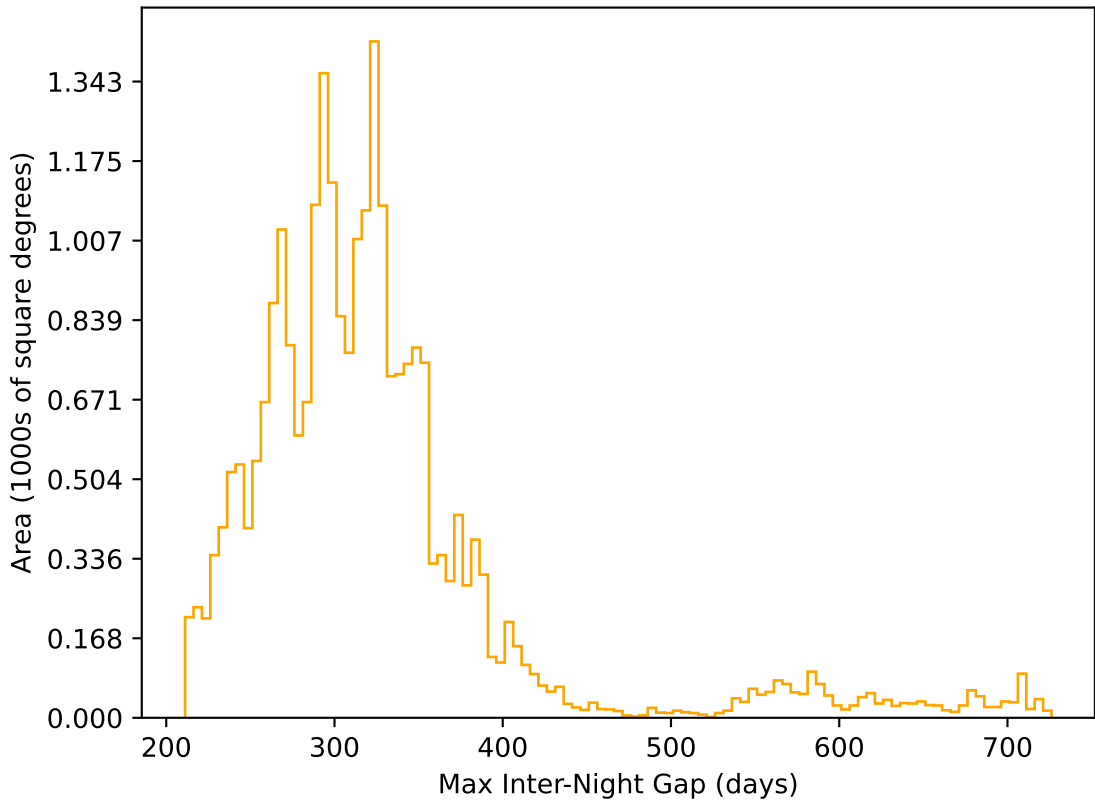
too_elab_r256_d2_griz_v3.4_10yrs All sky r band: Max Inter-Night Gap
